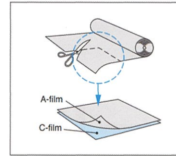
1. Cut the Prescale to the shape to be measured
