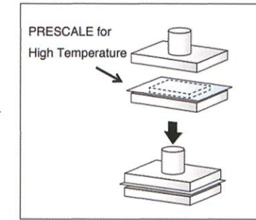
2. Place the cut Prescale in the measurement location and apply pressure
