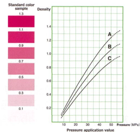
* Pressure chart for standard Prescale
